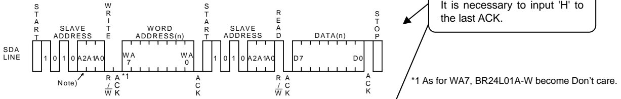
Figure 42. Random read cycle (BR24L01A/02/04/08/16-W)
